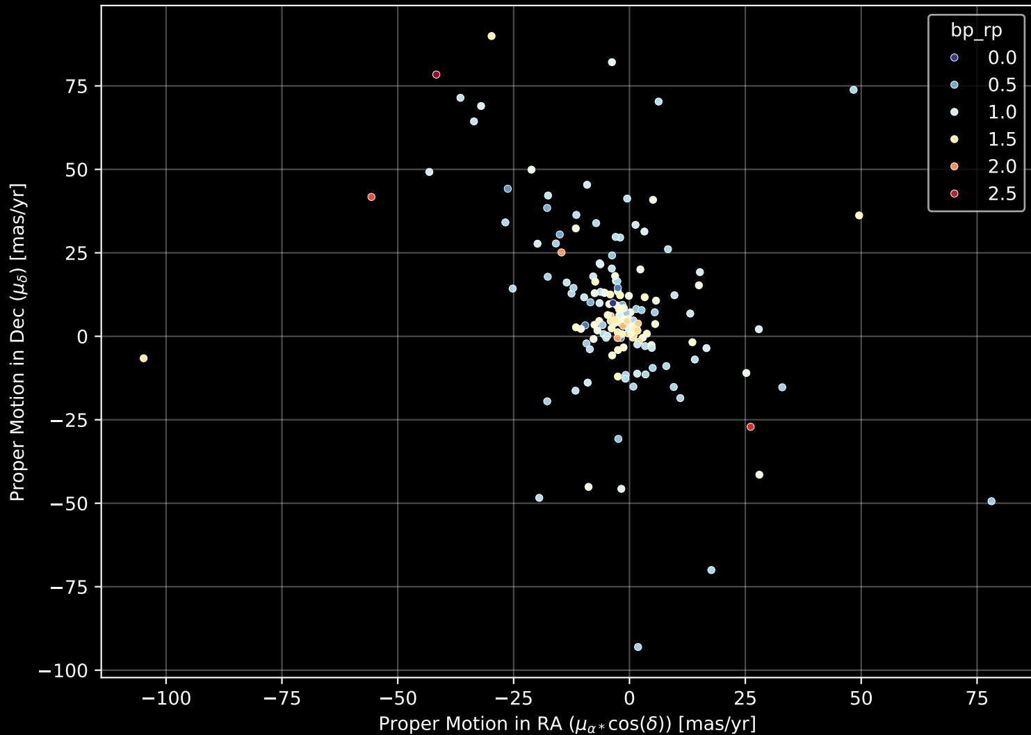
APOGEE DR17 Field: [269-20-O_TESS] Proper Motion Diagram (n= 166)
