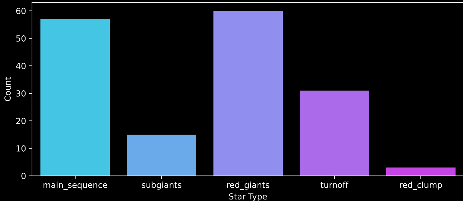
APOGEE DR17 Field: [269-20-O_TESS] Count plot of Star Type
