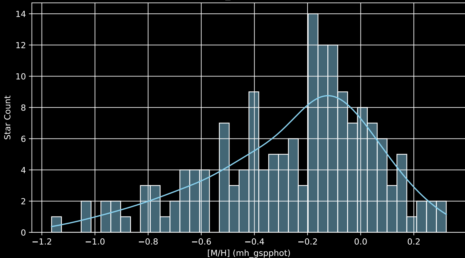
APOGEE DR17 Field: [269-20-O_TESS [M/H] (mh_gspphot) (n= 165)
