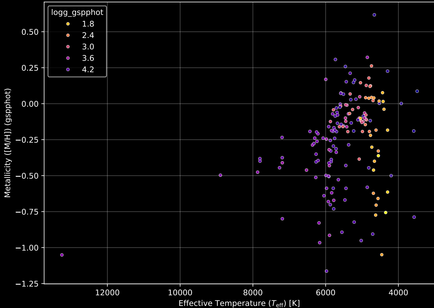
APOGEE DR17 Field: [269-20-O_TESS] Stellar Population Parameters (n= 166)
