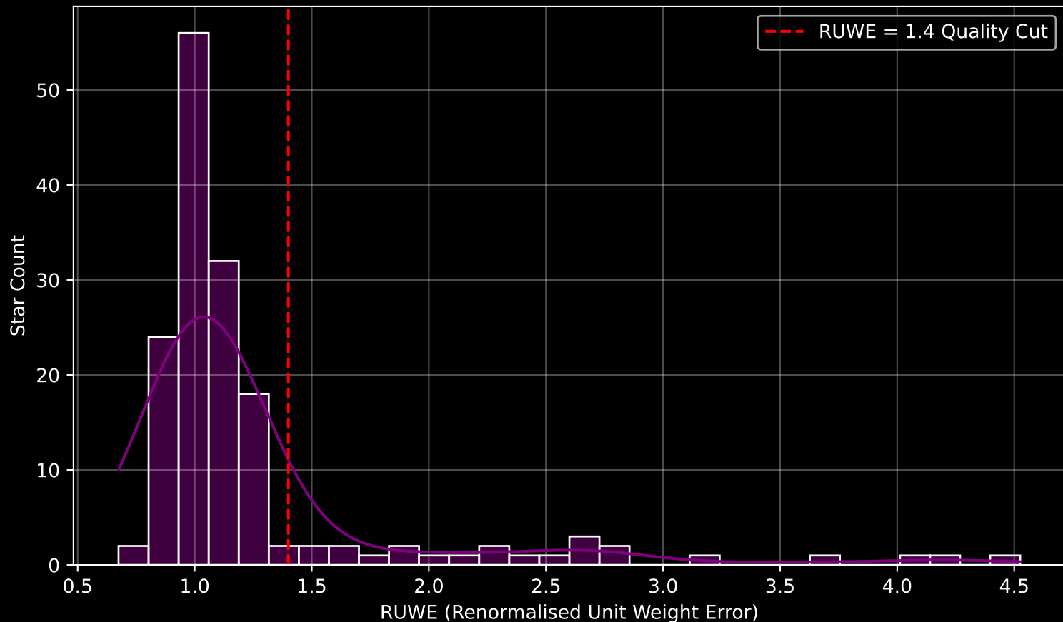
GAPOGEE DR17 Field [269-20-O_TESS] RUWE Distribution (n= 157)
