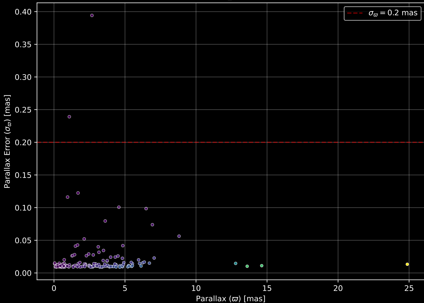
APOGEE DR17 Field: [269-20-O_TESS] Parallax Quality (n= 166)
